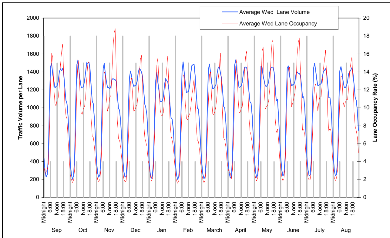
Figure 3-6. Wednesday Lane Volume Versus Occupancy
